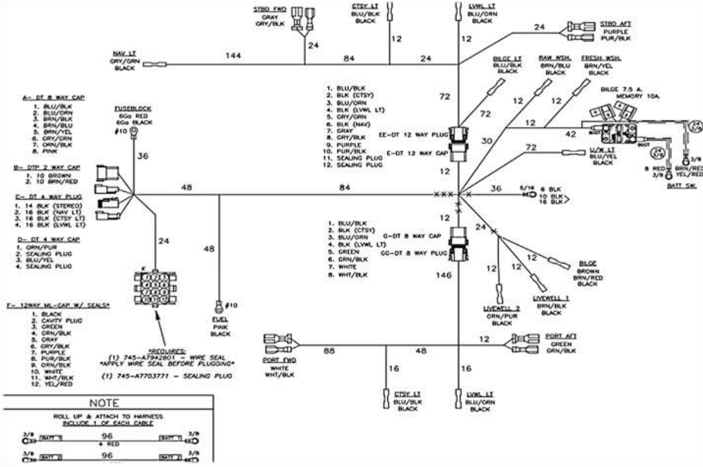
Fuse Panel
